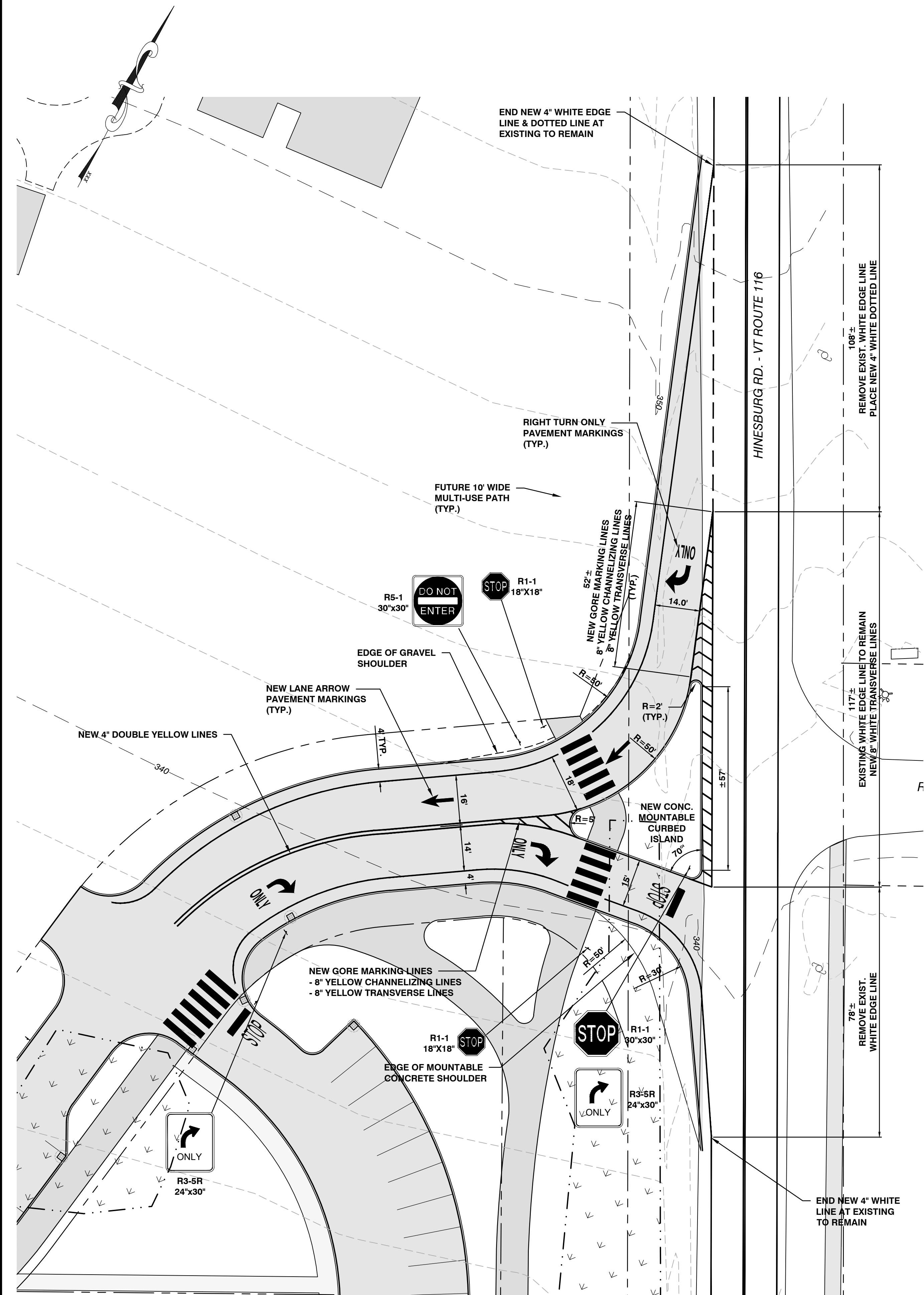
INTERSECTION LAYOUT
