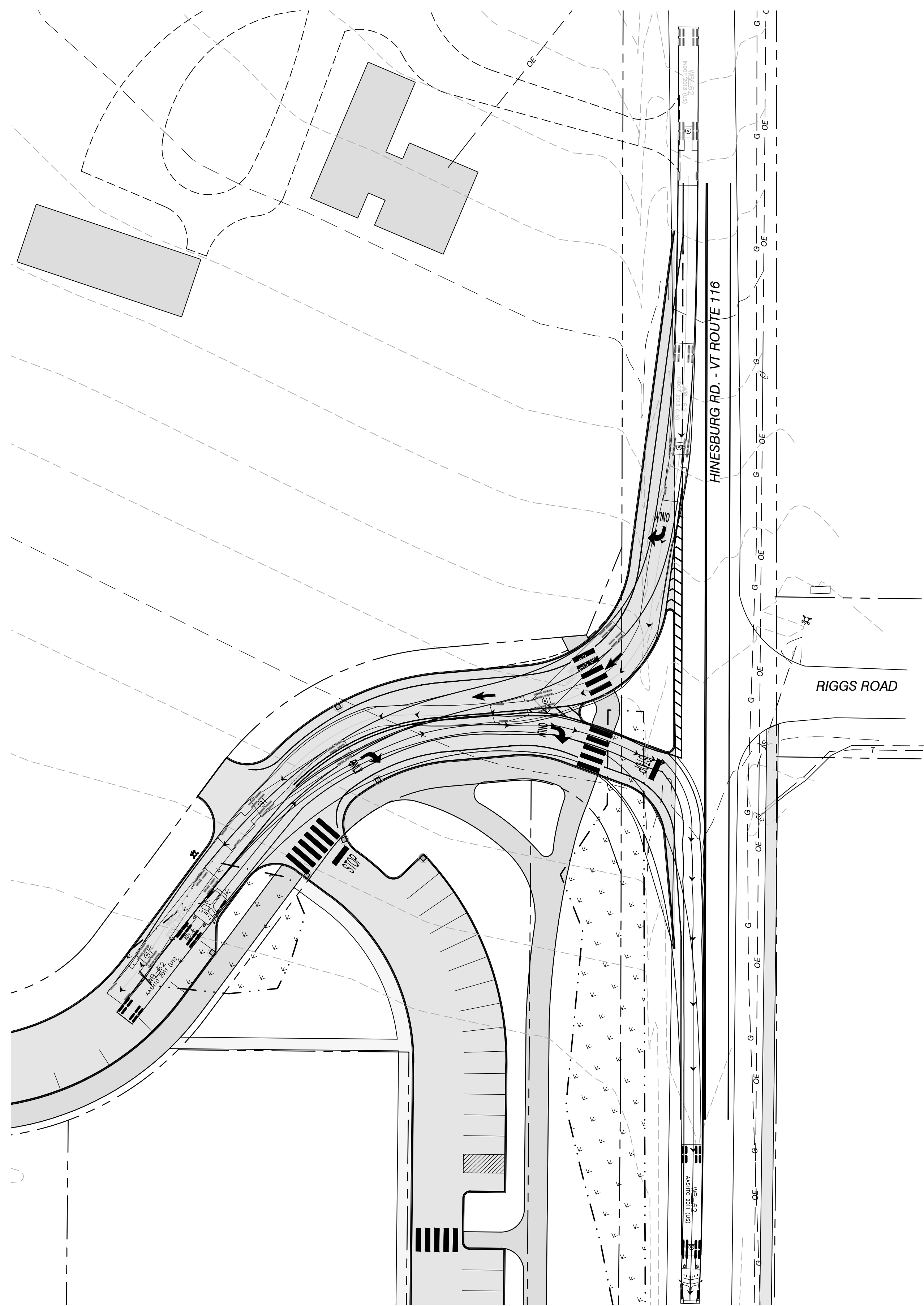
TRUCK TURNING MOVEMENTS
